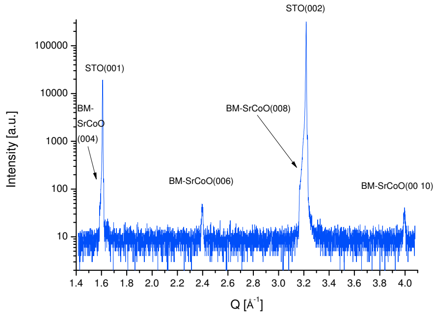
Figure 5.25: XRD measurement of sample 546-A. The Co/Sr ratio is 1.02.
