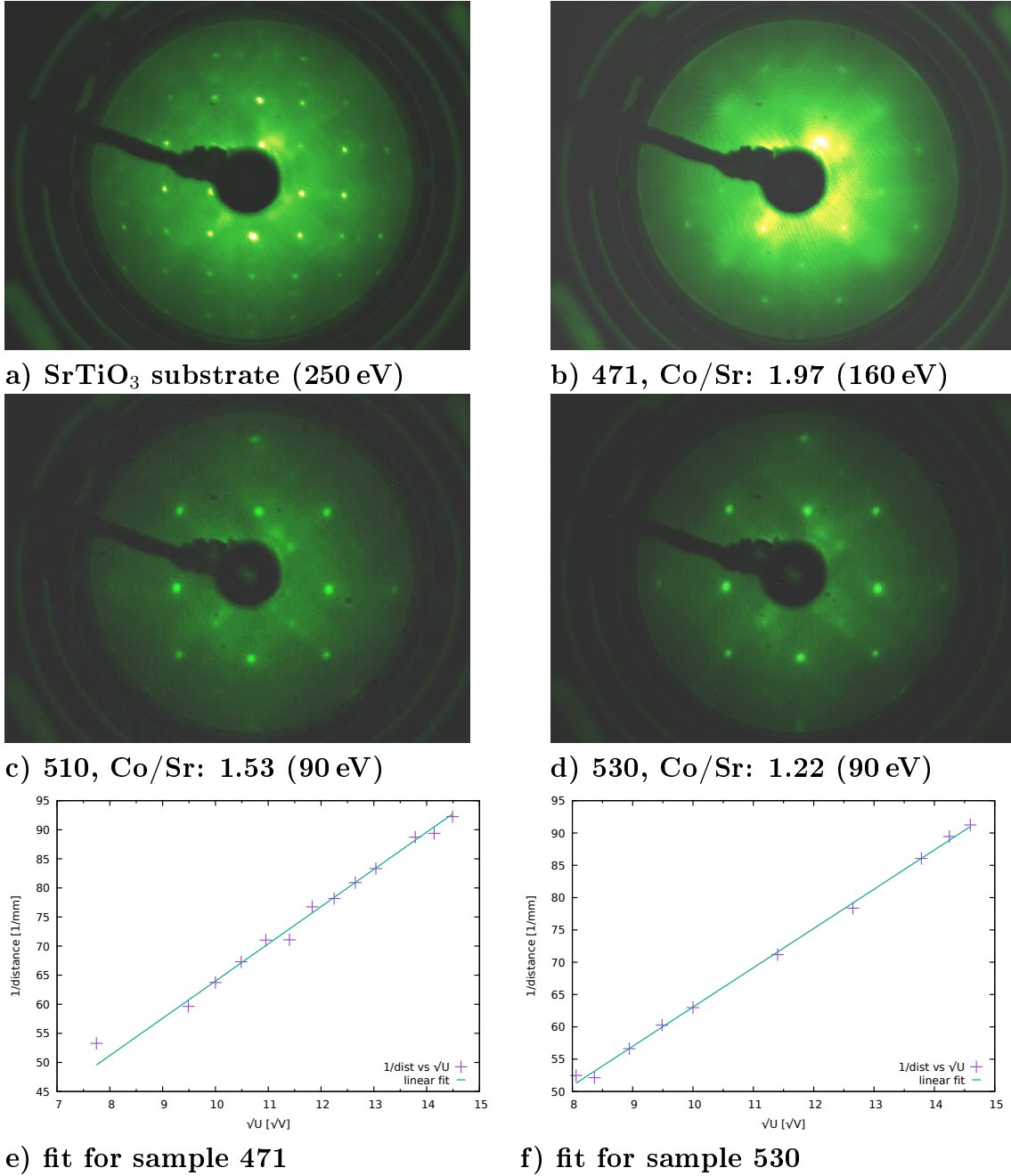
Figure 5.17: LEED images of an STO substrate at 250 eV (a) and different \text{SrCoO}_x samples with given Co/Sr ratio, sample 471 at 160 eV (b), sample 510 at 90 eV (c), and sample 530 at 90 eV (d). The brightness and contrast were optimized. In figs. (e) and (f) the inverted distance between Bragg-spots in the LEED images are plotted against the square root of the voltage according to equation 5.5. This is shown for sample 471 (e) and 530 (f), as an example. The resulting lattice constants are 5.7 Å and 5.6 Å, respectively.
