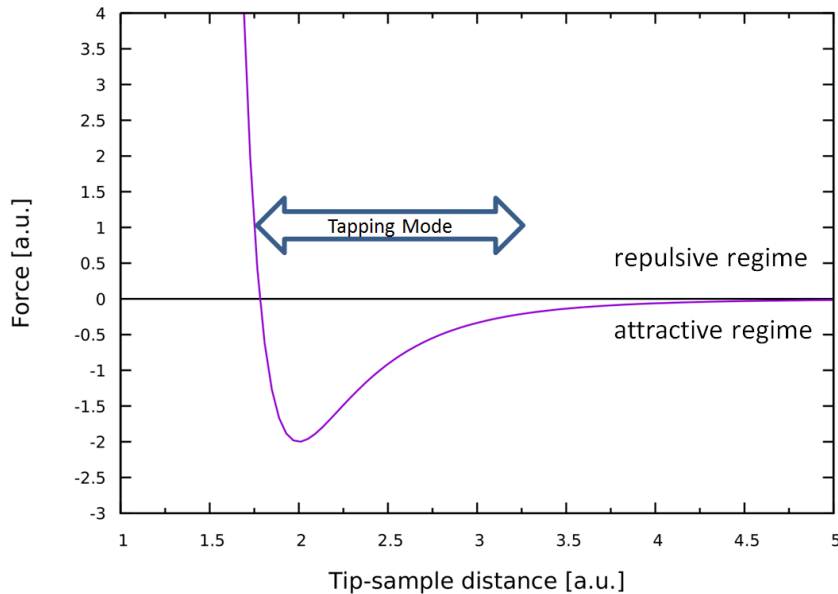
Figure 3.2: Lennard-Jones potential.
