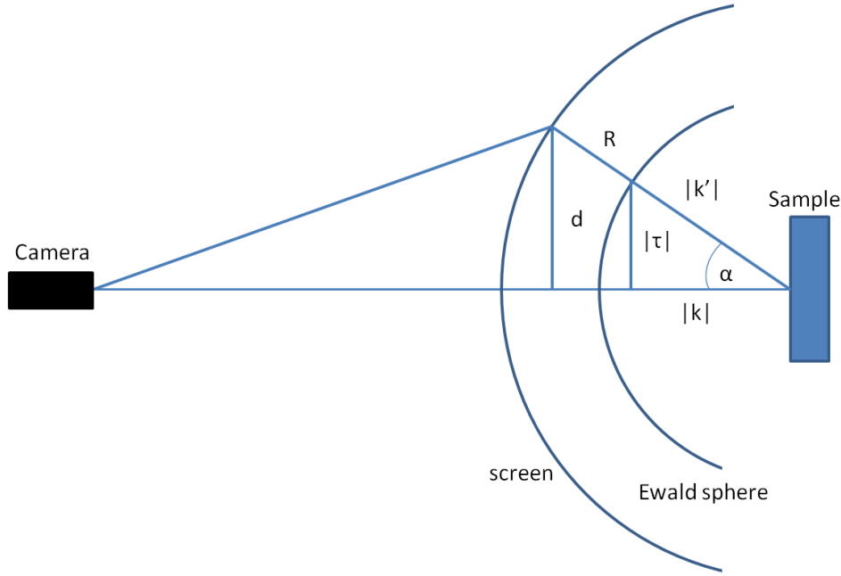
Figure 3.3: LEED geometry with Ewald sphere.
