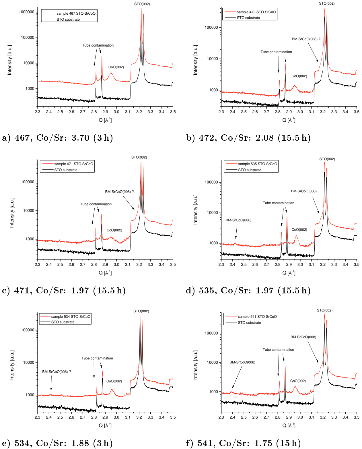
Figure 5.26: XRD measurements in decreasing order of Co/Sr ratio for samples. The measurement time is given in brackets.
