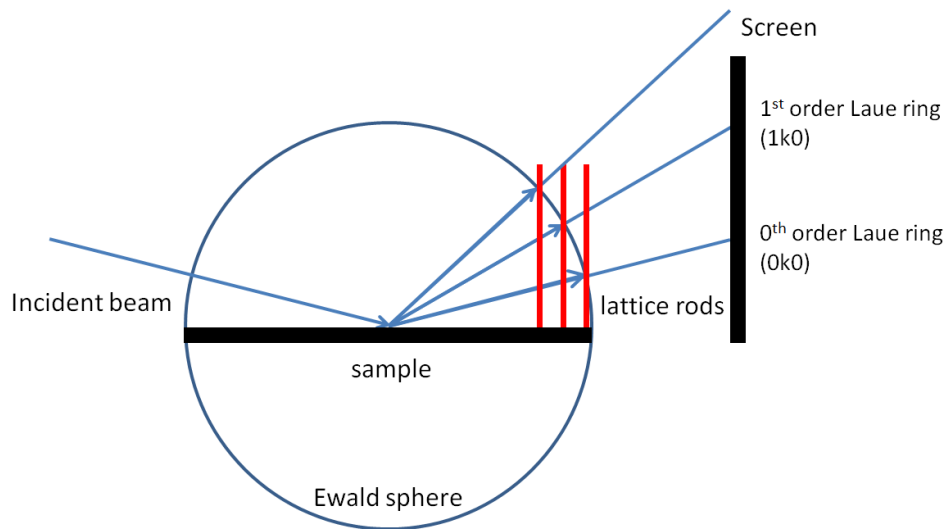
Figure 3.4: Ewald construction for RHEED geometry.
